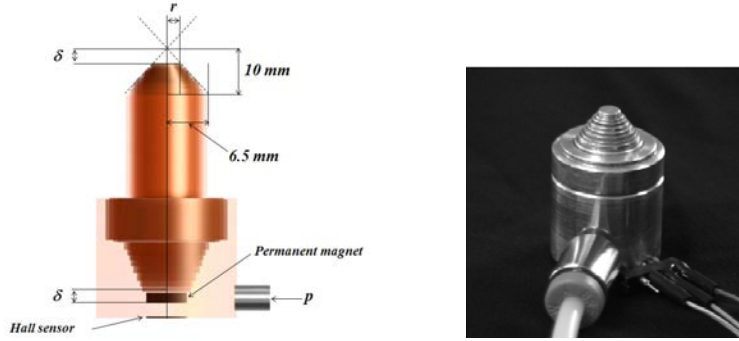
Figure 5.4: Geometry (left) and appearance (right) of the softness display. The prototype has a max. height of 33 mm and a diameter of 13 mm.
