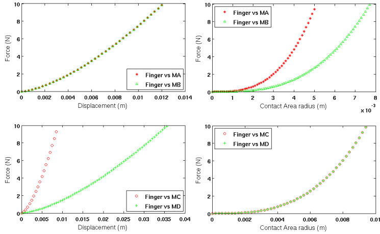
Figure 5.3: Comparison of the force-displacement (left column) and force-area (right column) curves for finger-object contacts. In the first row, two objects M_A and M_B have parameters E_A = 10^6 \text{ N/m}^2 , R_A = 2.5 \text{ mm} , E_B = 1.5 \cdot 10^5 \text{ N/m}^2 , R_B = 7.3 \text{ mm} , which satisfy relation 5.4. In the second row, two objects M_C and M_D have parameters E_C = 2 \cdot 10^5 \text{ N/m}^2 , R_C = 30 \text{ mm} , E_D = 2 \cdot 10^4 \text{ N/m}^2 , R_D = 3 \text{ mm} , satisfying relation 5.5.
