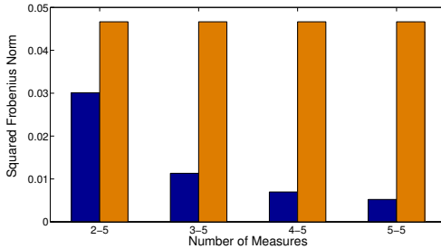
Figure 4.13: Squared Frobenius norm for the a posteriori covariance matrix of H_s with m = 5 measures, and H_d^* with m = 2, 3, 4, 5 measures, in case of noisy measures.
