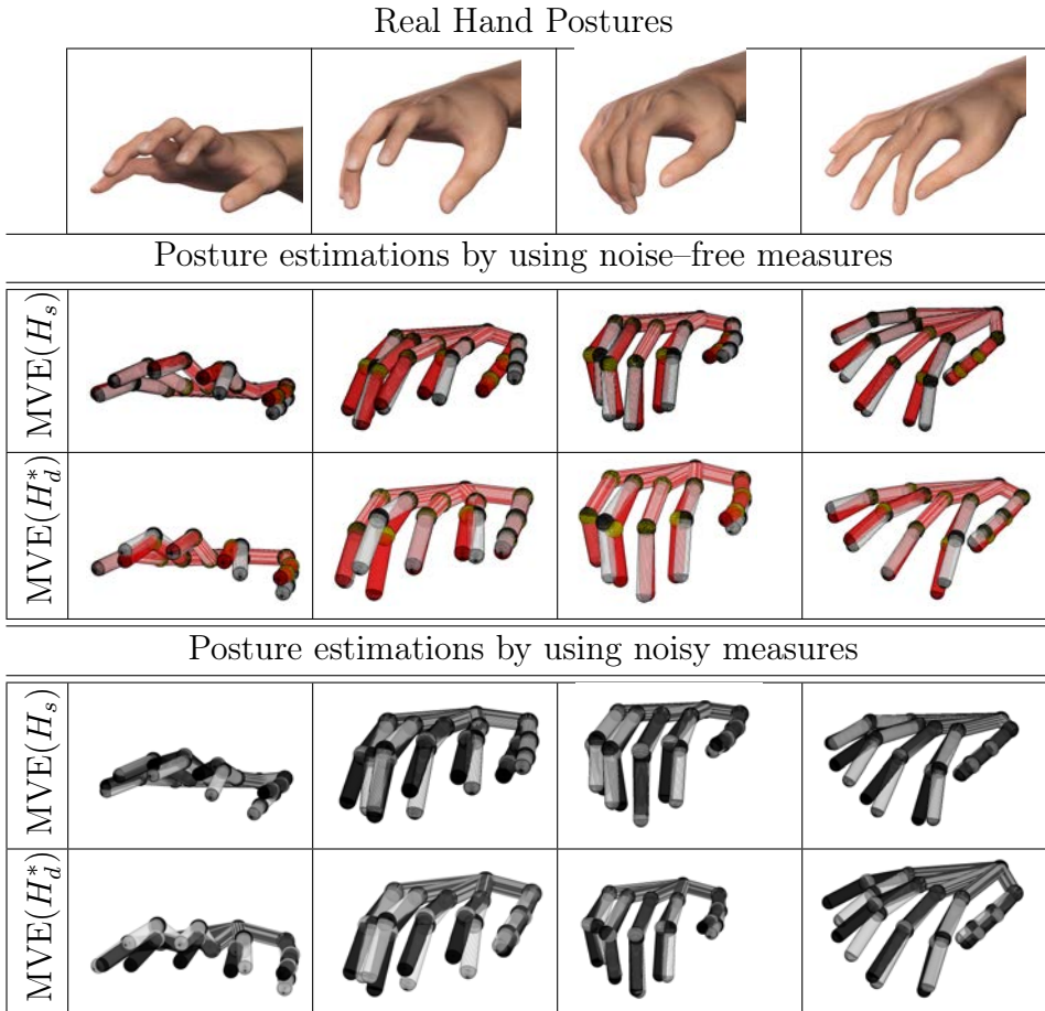
Figure 4.11: Hand pose reconstructions MVE algorithm by using matrix H_s which allows to measure TM , IM , MM , RM and LM and matrix H_d^* which allows to measure TA , MM , RP , LA and LM (see figure 4.1)– in noise-free case – and TA , MM , MP , LM and LP – in case of noise. In color the real hand posture whereas in white the estimated one.
