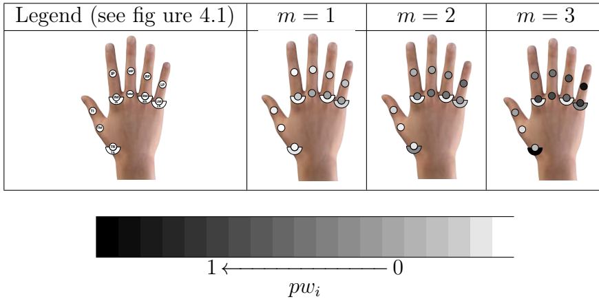
Figure 4.6: Optimal continuous sensing distribution for m = 1 , i.e. the first PC of P_o , for m = 2 , i.e. the first two PCs of P_o and for m = 3 , i.e. the first three PCs of P_o . The greater is the weight pw_i of the joint angle in the optimal measures, the darker is the color of that joint. For visualization purposes, I assume the weight of the i -th joint in the optimal measures given as pw_i = \sum_{k=1}^m |h_{k,i}| , where h_{k,i} is the (k, i)^{th} entry of matrix H , normalized w.r.t. the maximum value of pw_i . For example, for m = 3 , weight of LA joint is 0.53, whereas for LM joint is 0.74 and the maximum value is for TA joint.
