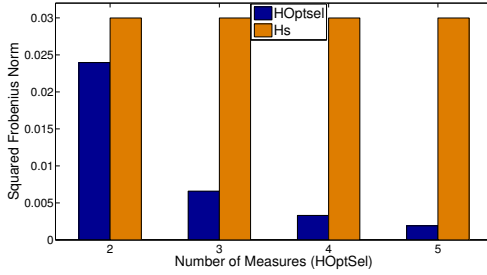
Figure 4.12: Squared Frobenius norm for the a posteriori covariance matrix of H_s with m = 5 measures, and H_d^* with m = 2, 3, 4, 5 measures, in case of noise-free measures.
