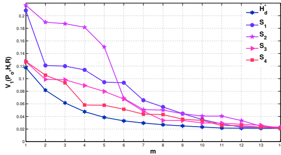
Figure 4.9: Squared Frobenius norm of the a posteriori matrix with noisy measures for the discrete case. The optimal measurement matrix H_d^* is compared with 4 random matrices adding the same quantity of noise (with standard deviation of 7^\circ ).
