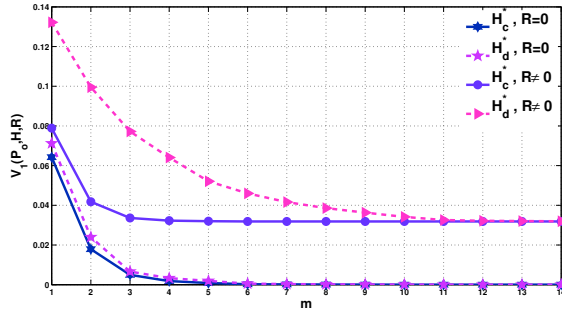
Figure 4.8: Squared Frobenius norm of the a posteriori matrix with noise-free and noisy measures (with standard deviation of 7^\circ ) for both H_c^* and H_d^* .
