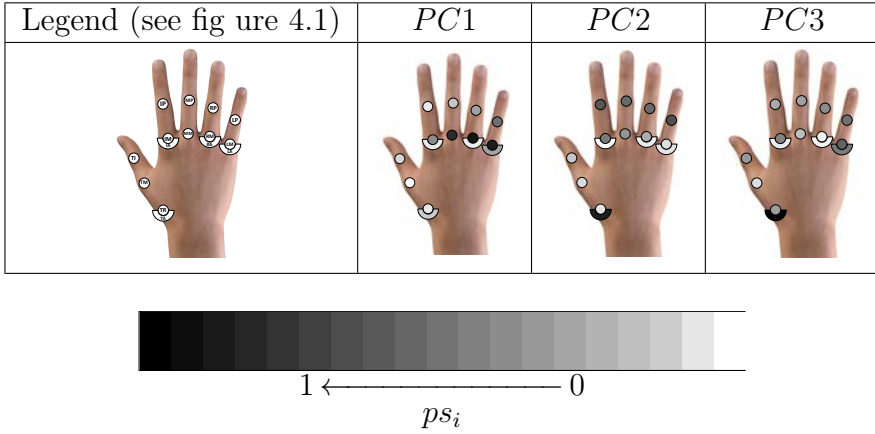
Figure 4.7: Optimal continuous sensing distributions for the first PCs of P_o ( PC1 , PC2 , PC3 ). The greater is the absolute coefficient ps_i of the joint angle in the PC, the darker is the color of that joint. For visualization purposes, I assume the coefficient of the i -th joint in the PC to be normalized w.r.t. the maximum absolute value of the coefficients achieved across PC1 , PC2 , PC3 .
