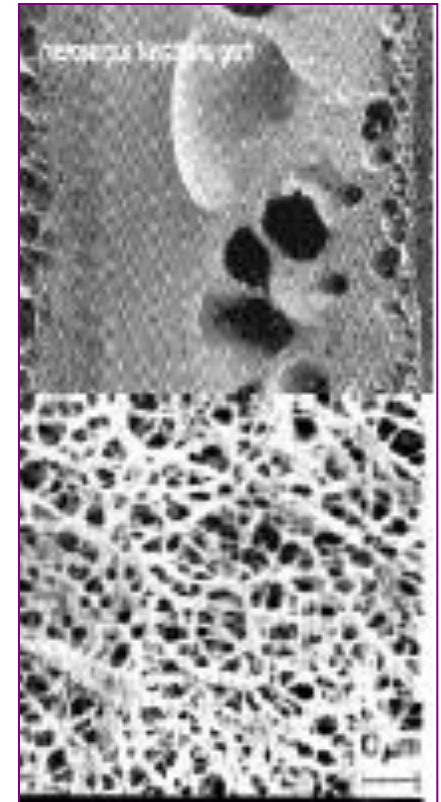
Wall with variable porosity obtained by filament winding
