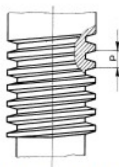
Profilo trapezoidale (acme)
